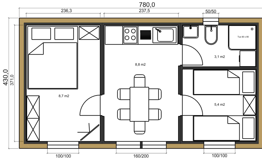
Floor plan
